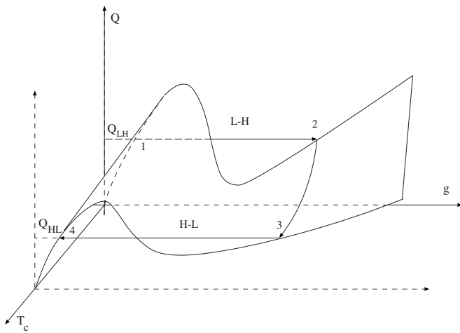
FIG. 10. Hysteresis phenomenon in the L–H transition in a three-dimensional parameter space that also includes the core temperature; first, the L–H transition (1–2) occurs at a relatively low rate since the system starts from the L mode. When the gradient g builds up at the edge, increases (2–3) lowering thus the heating requirements for transitions. Then, if the heating Q decreases to its Maxwell value, the reverse transition occurs at lower Q than the forward one.
